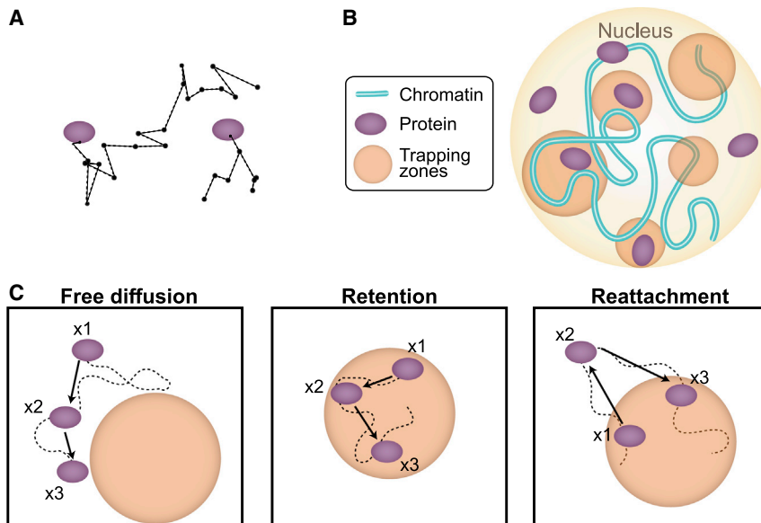
Figure 7. A Model for Nuclear Protein Dynamics Based on Retention and Reattachment
