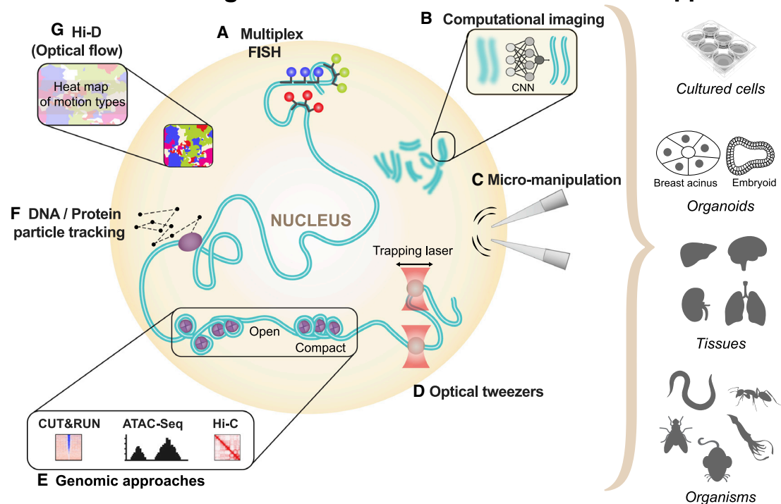
Figure 1. An Overview of Techniques for Exploring Chromatin Discussed in This Review
