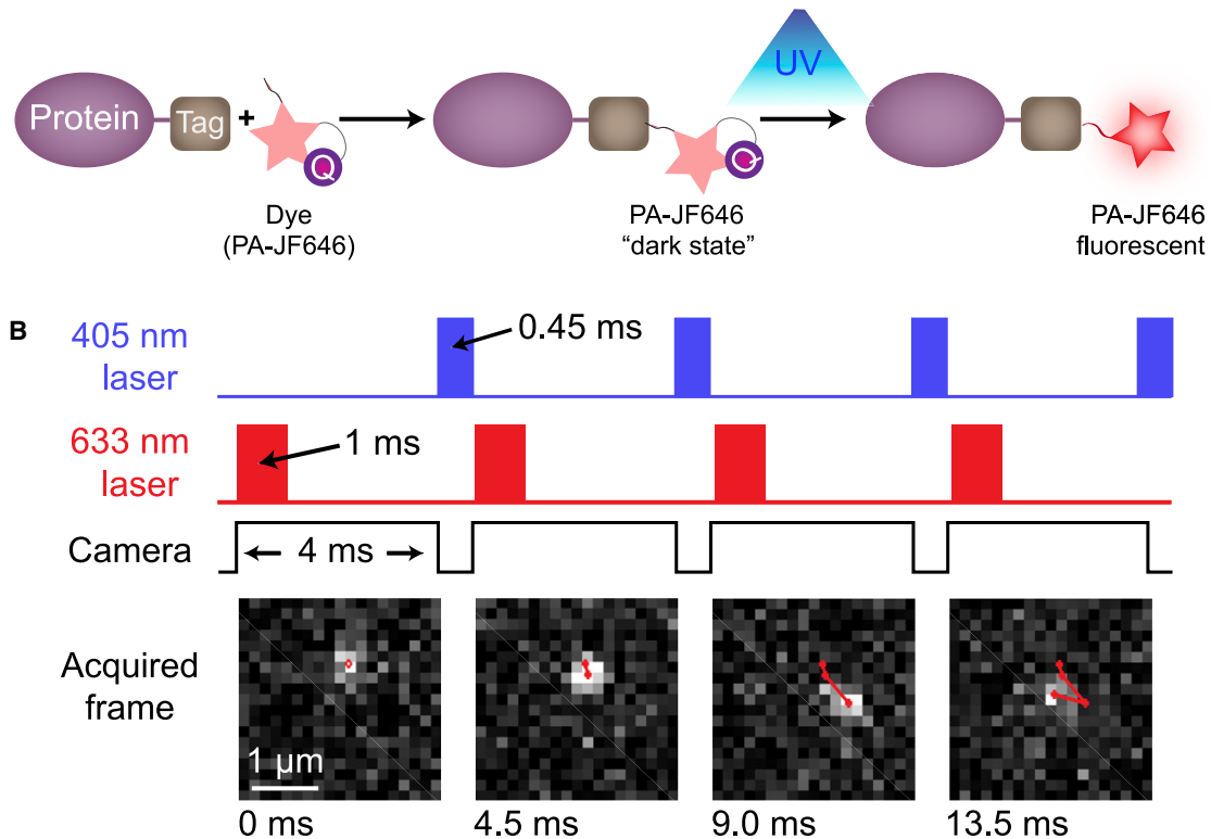
Figure 4. Stroboscopic Photo-activation Single-Particle Tracking
